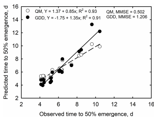
Figure 2. Comparison of observed and simulated days to time to 50% seed emergence (t50%) of the growing degree day (GDD) and quadratic (QM) models for soybean seed emergence across a wide range of genetic, experimental, and environmental conditions.
