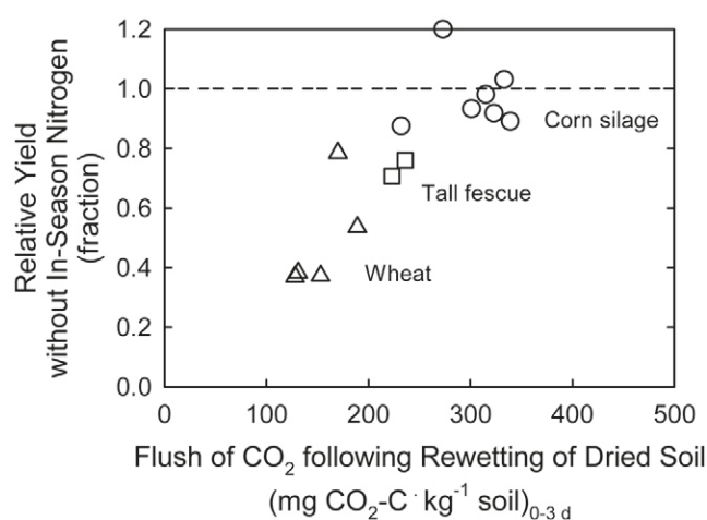
Fig. 4. Preliminary results relating the flush of \text{CO}_2 to relative crop yield response to N fertilizer (yield without in-season N compared with yield with highest N rate) (A.J. Franzluebbers, unpublished data; collaboration with S. Gibson on wheat [ Triticum aestivum L.], C.D. Teutsch on tall fescue [ Schedonorus arundinaceus (Schreb.) Dumort.], and J. Cline, A. Lipscomb, T. Mize, and R.S. Shoemaker on corn [ Zea mays L.] silage).
