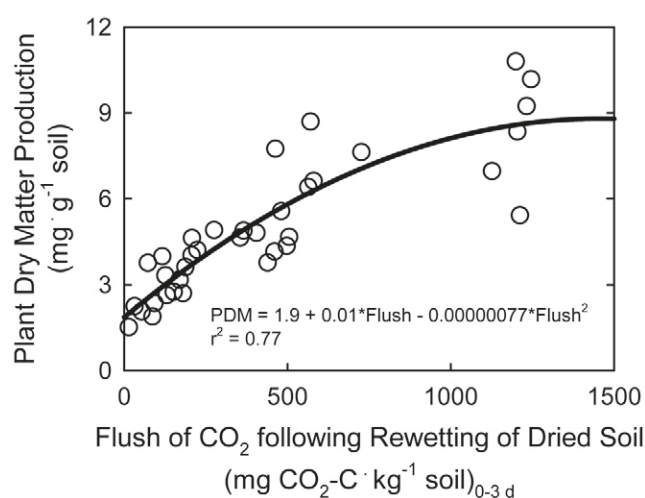
Fig. 3. Preliminary results relating the flush of \text{CO}_2 to plant dry matter production under greenhouse conditions (M.R. Pershing, unpublished data). Soils (Typic Kanhapludults) were samples from a long-term pasture–crop rotation study in Watkinsville, GA (Franzluebbers and Stuedemann, 2015).
