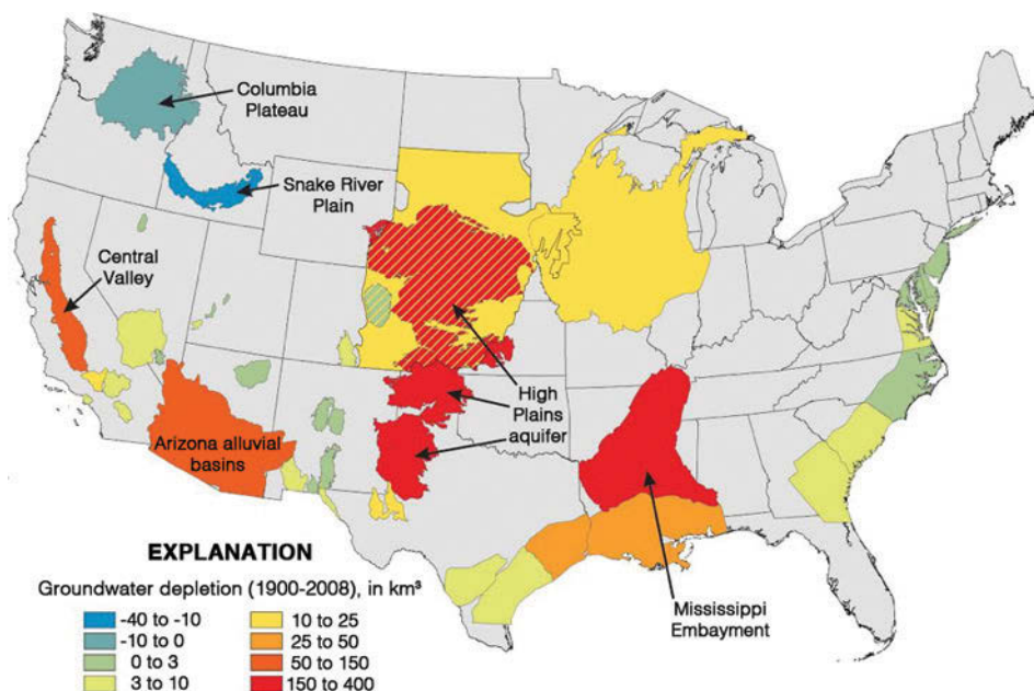
Figure 4. Cumulative long-term volumetric groundwater depletion in the United States during 1900–2008 in km³ (modified from Konikow [2013]). Hachured areas are where a shallow aquifer overlies a deeper aquifer.
