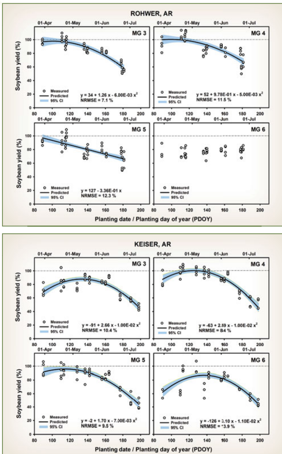
Figure 2: Soybean relative yield versus planting date by MG from a three-year study at Rohwer, Arkansas (top panel) and Keiser, Arkansas (bottom panel). The open symbols indicate observed data, the solid line shows the estimated relative yield for each MG (equation provided in the figure), and the blue shaded area represents the 95 percent confidence interval in the prediction of the relative yield model. The normalized root mean square error (NRMSE) is provided as a measure of the goodness of the model fit with lower values indicating a better fit.
