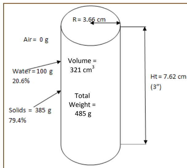
Figure 11. Soil core dimensions, volume, and weight (by component) Example 1.
