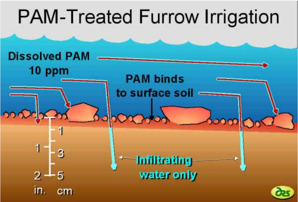
Figure 2 Schematic depiction of PAM deposition from treated water onto soil aggregates in the surface few millimeters of soil in an irrigated furrow.
