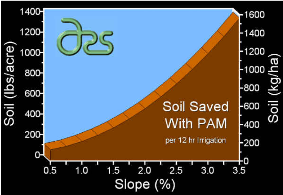
Figure 3 Estimate of soil saved as a function of slope for twelve hour irrigations on Portneuf silt loam using inflows of 23-38 L/min for an approximately 200 meter long field.
