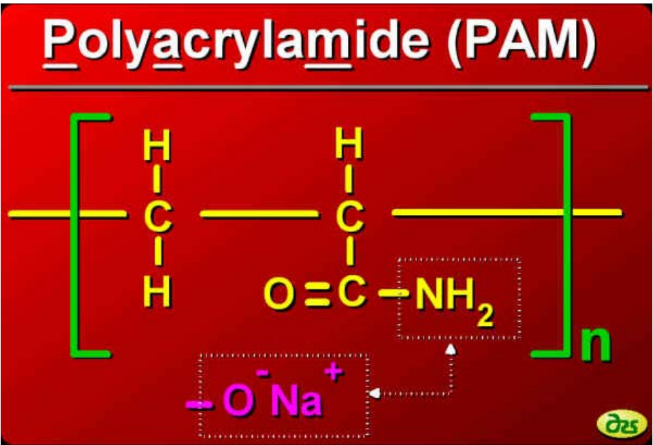
Figure 1 Depiction of an individual acrylamide monomer component as found in a polyacrylamide molecule. Substitution of the sodium formate functional group for the amide group, as occurs in about one in five polymer units is shown. This is the substitution that, when sodium dissociates from the copolymer chain, provides a net negative charge on the "PAM" molecule.
