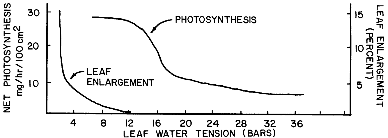
Figure 4. Rates of leaf enlargement and net photosynthesis of soybeans at various leaf-water potentials (after Boyer).
