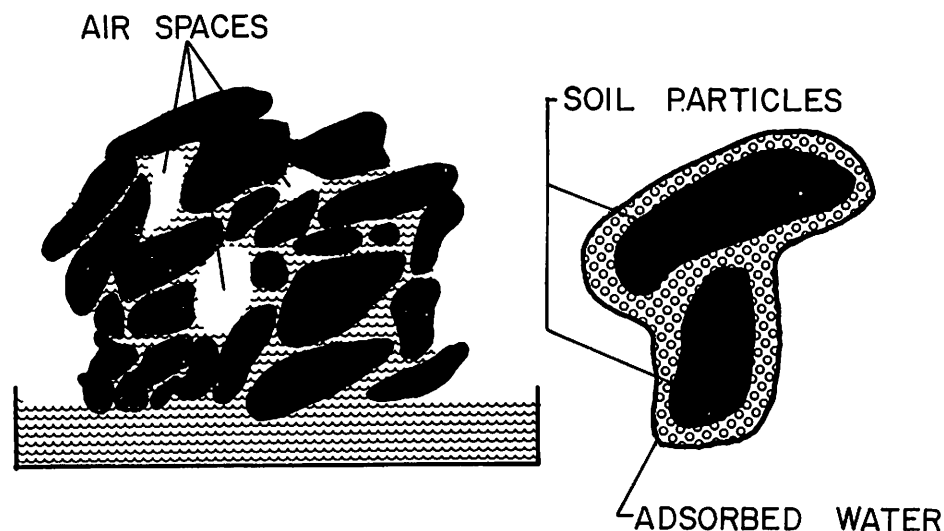
Figure 1. (Left) Diagram of soil particles with saturated zone at bottom. Drainage has allowed air to enter larger pore spaces near surface.
